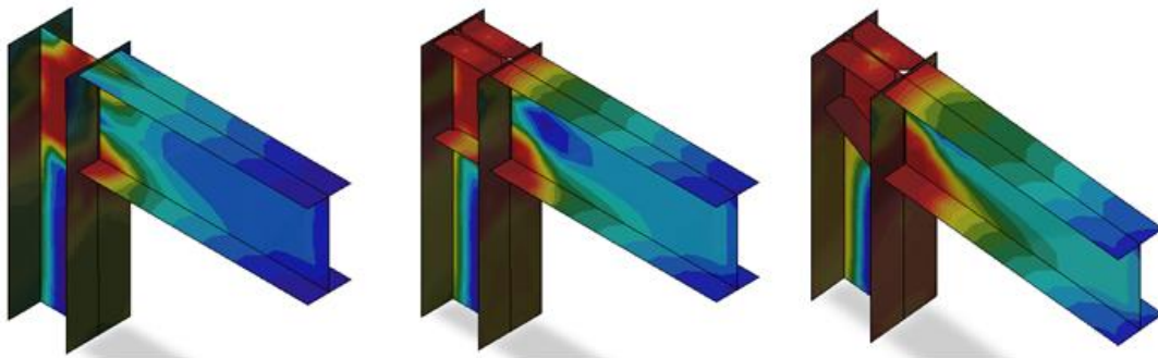
Figure 5: Influence of the shear stiffener to eaves moment connection; from left 46,5 KNm; 61,3 kNm; and 73,0 kNm
