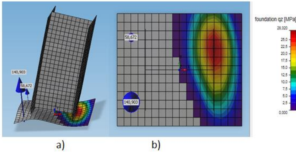
Figure 7: Base plate loaded by general moment a) deformed shape, b) stress in contact area
