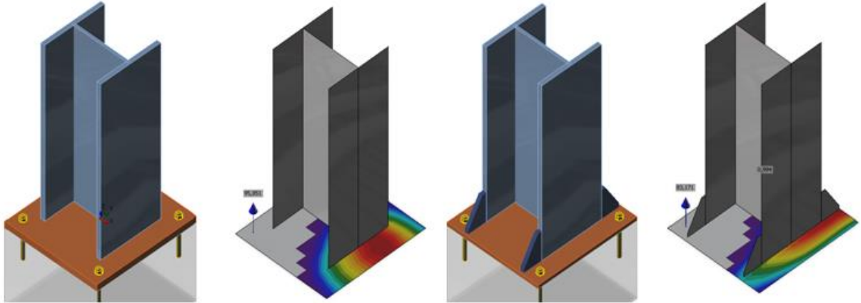
Figure 6: Stress in concrete under unstiffened base plate 35 mm (left) and stiffened base plate 22 mm loaded by general moment (right)
